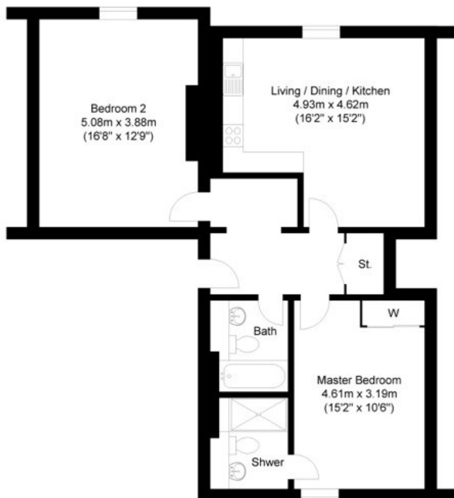
First Floor Approximate 78.90 sq meter (849.0 sq feet)
